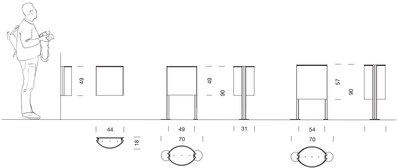
Rambla wall attachable litterbin
