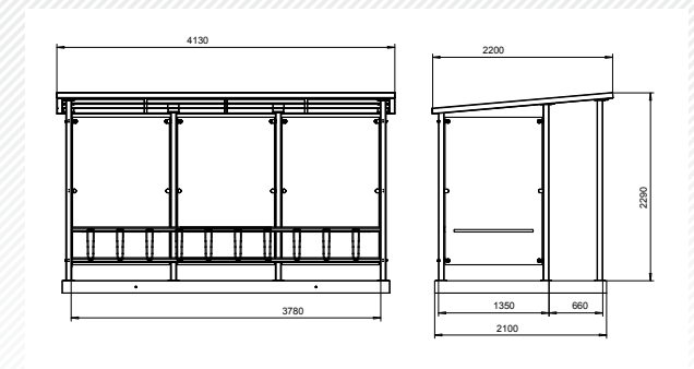
Bicycle shelter
