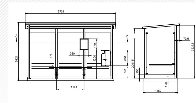
Bus shelter
